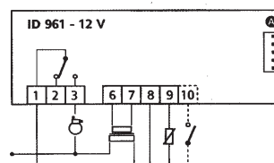
ID 961/A PTC
